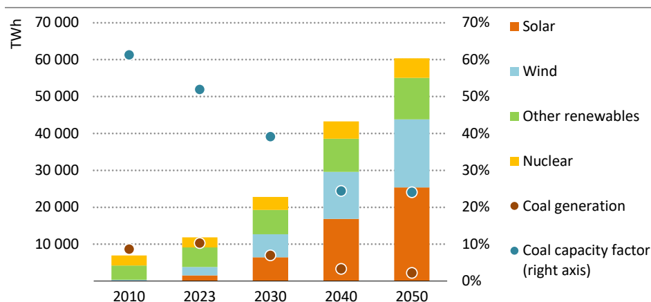
Figure 2.4 ▶ Low-emissions power generation by source and average capacity factor of coal-fired power plants in the APS, 2010-2050
